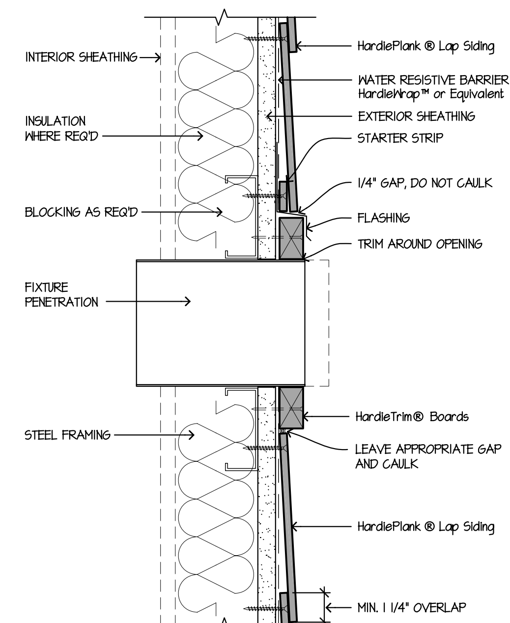
7 FIXTURE PENETRATION SCALE: 3/8"=1'-0"
