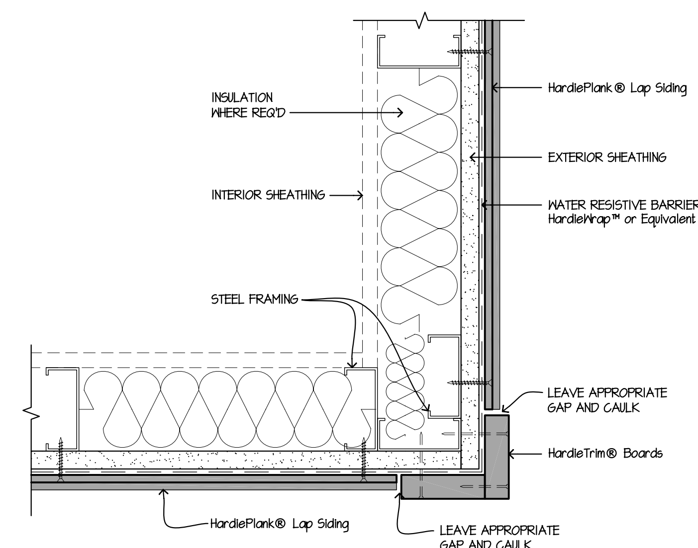
2 OUTSIDE CORNER SCALE: 3/8"=1'-0"
