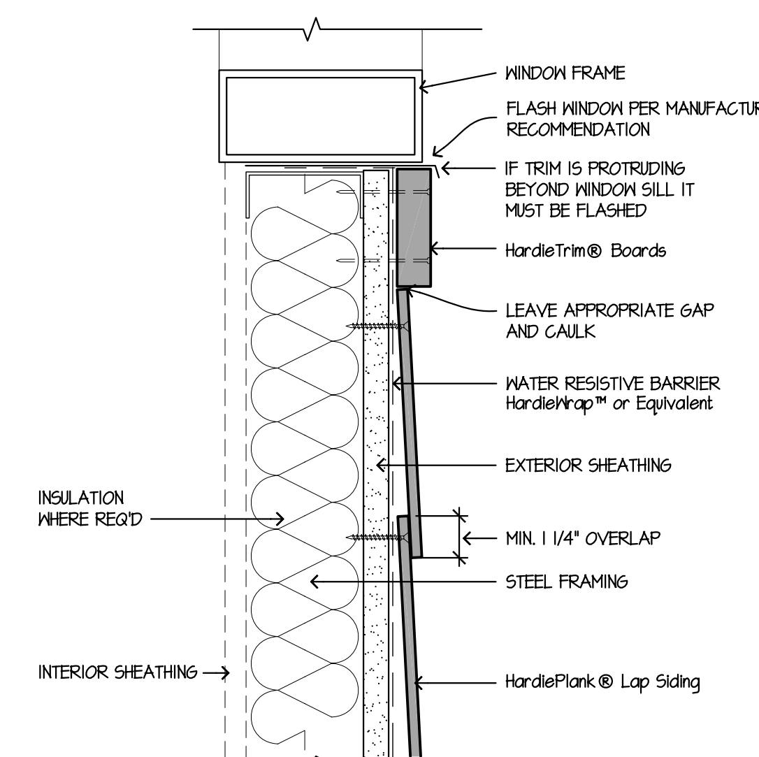
5 HORIZONTAL LAP VIEW SCALE: 3/8"=1'-0"
