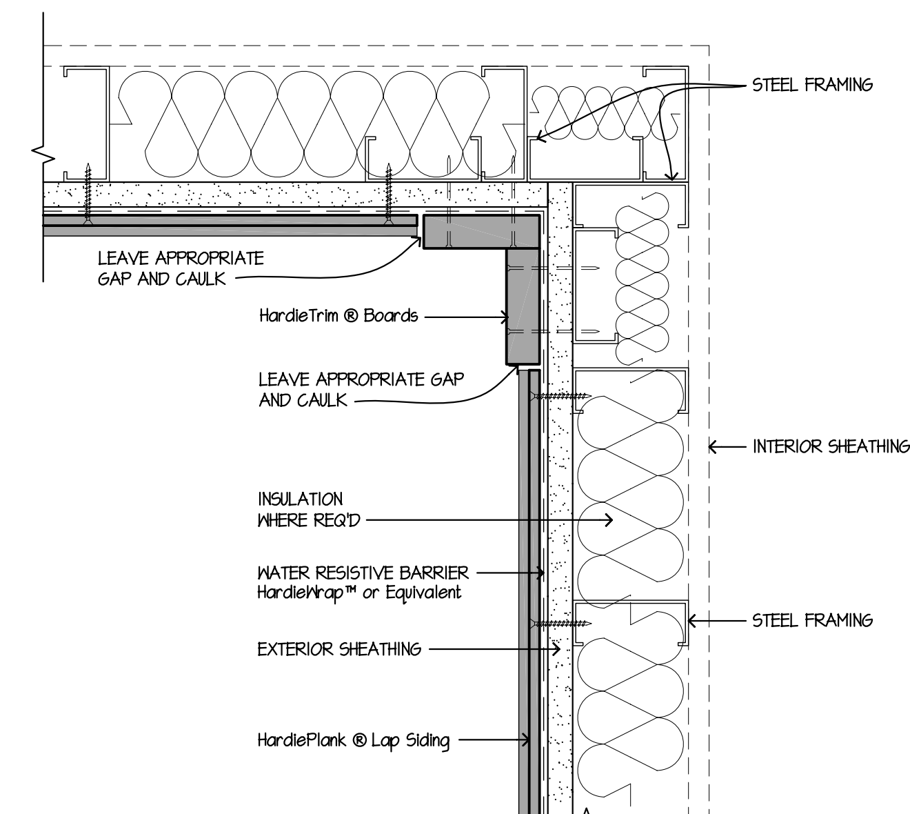
1 INSIDE CORNER SCALE: 3/8"=1'-0"
