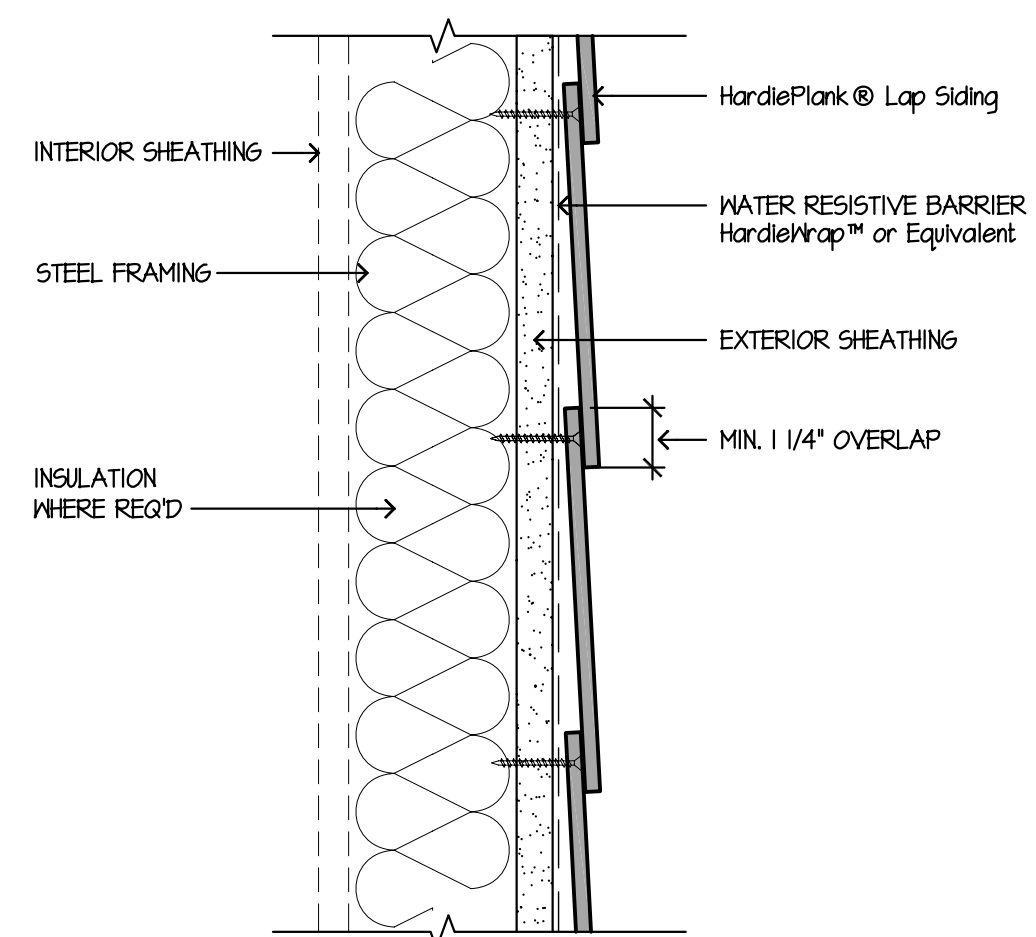
5 HORIZONTAL LAP VIEW SCALE: 3/8"=1'-0"
