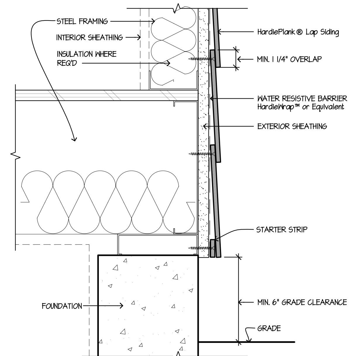
6 GRADE CLEARANCE SCALE: 3/8"=1'-0"
